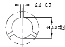
ARBOR HOLE DETAIL A SCALE 2:1
